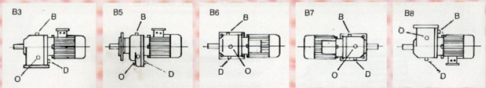
D - Drain plug O - Oil level indicator B - Breather plug and oil filler
