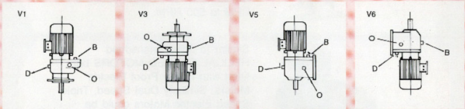
D - Drain plug O - Oil level indicator B - Breather plug and oil filler
